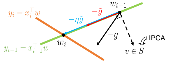
Fig. 1: An illustration of ORFit in the parameter space for a linear model. The parameter w_{i-1} fits the previous datapoints \{(x_k, y_k)\}_{k=1}^{i-1} . The set S (which is updated incrementally) consists of the directions moving towards which causes the most change in the predictions on previous data, and thus, moving orthogonal to S keeps the predictions intact. Given a new datapoint (x_i, y_i) , projecting its corresponding gradient g to the orthogonal complement of the subspace spanned by S yields the new update direction \tilde{g} . ORFit finds a new parameter w_i along the direction of -\tilde{g} which fits the new datapoint (x_i, y_i) within a single step, while still fitting the previous data \{(x_k, y_k)\}_{k=1}^{i-1} .
